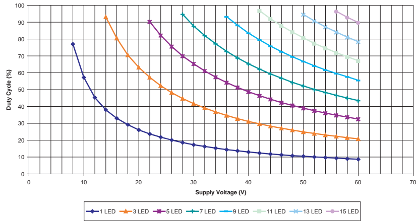
ZXLD1360 Duty Cycle L=150μH
